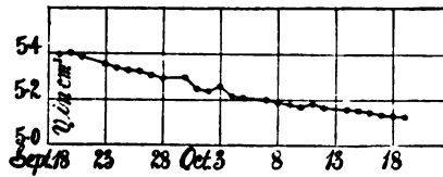
FIG. 27.—Chart showing loss of standard volumes of gas in diver in lapse of days. Diffusion of air through \text{CaCl}_2 solution.
